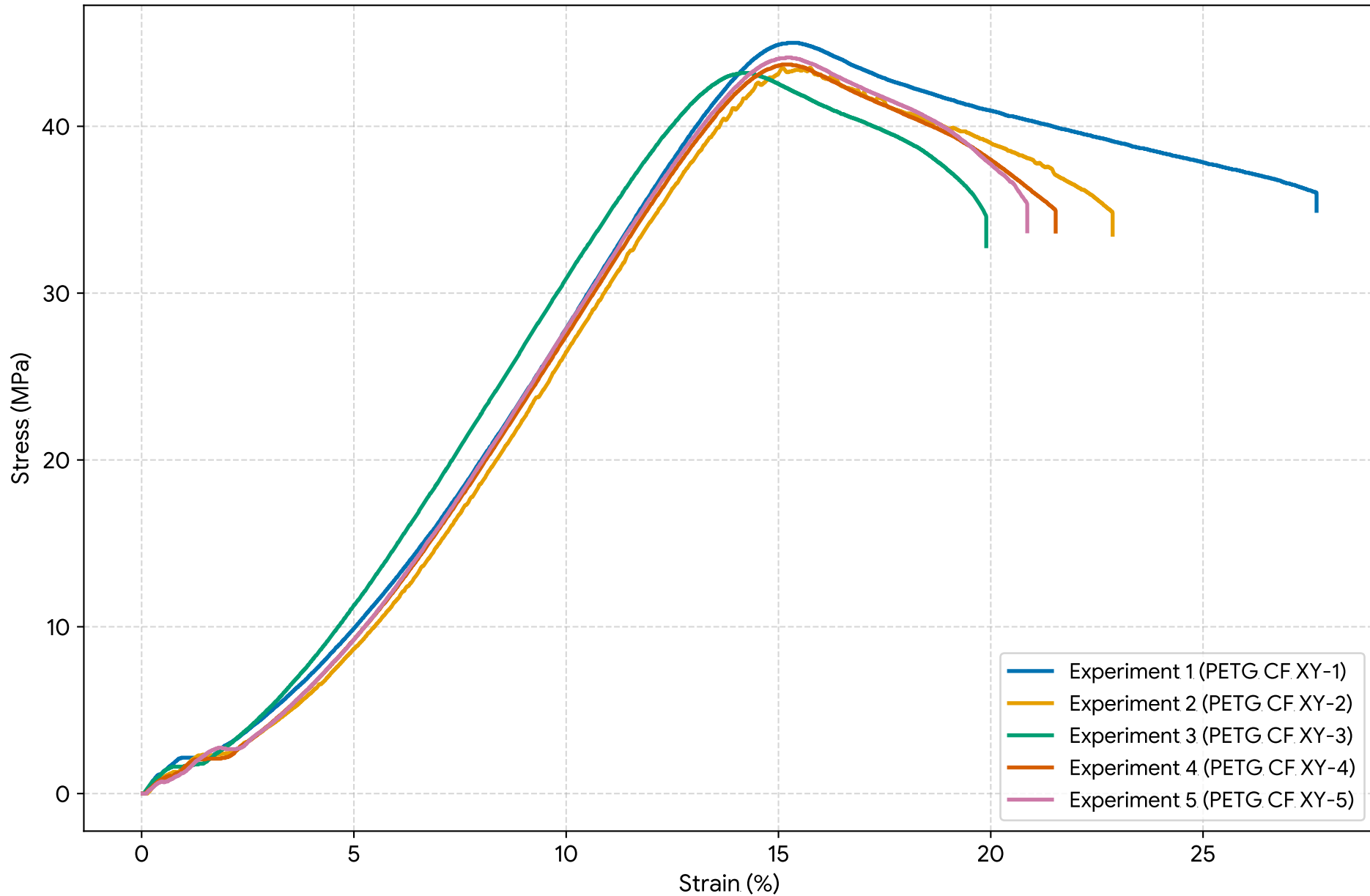
Stress-Strain Curves for PETG CF XY (5 Experiments)
